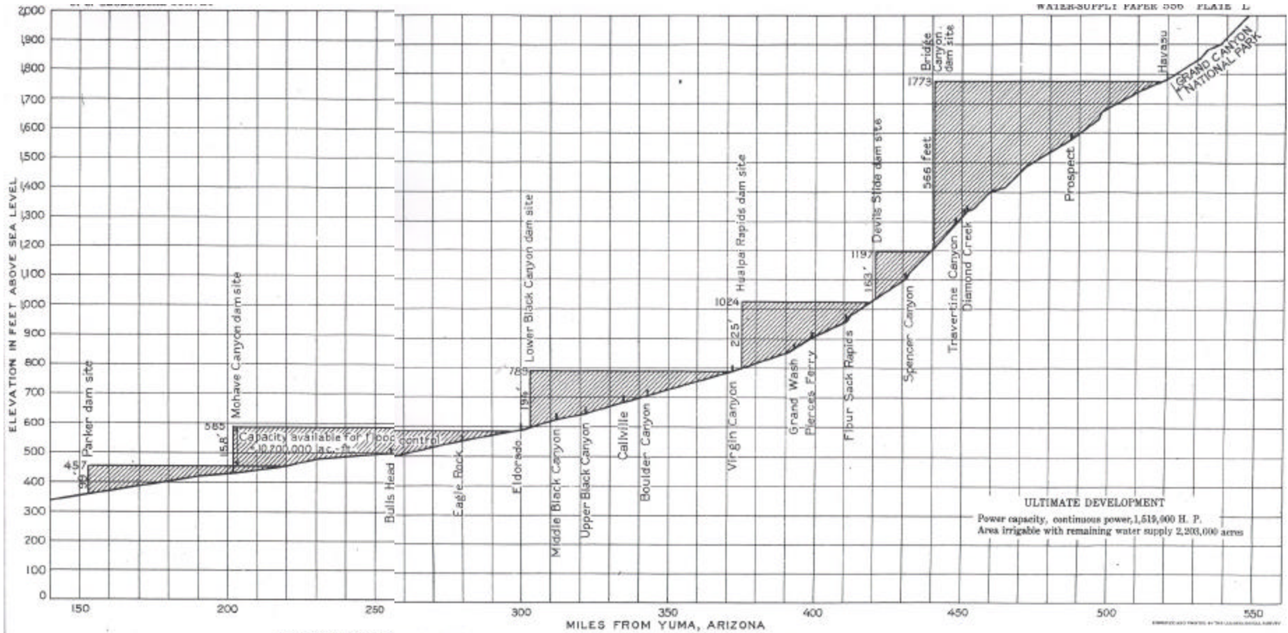
PLAN OF DEVELOPMENT OF COLORADO RIVER BETWEEN GRAND CANYON NATIONAL PARK AND PARKER, ARIZONA Names below profile represent alternative dam sites
